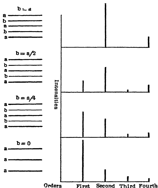
Fig. 76.—Relation between Densities of alternate Planes of Atoms and Intensities of Reflection Orders.
